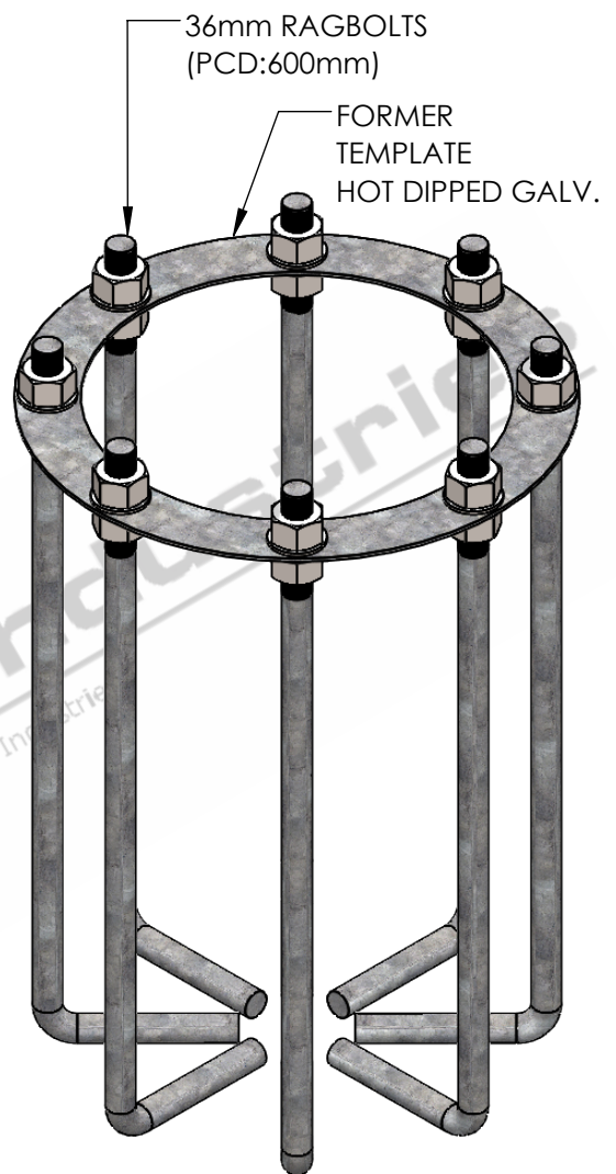
ISOMETRIC VIEW
