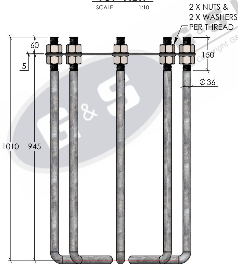
TOP VIEW
