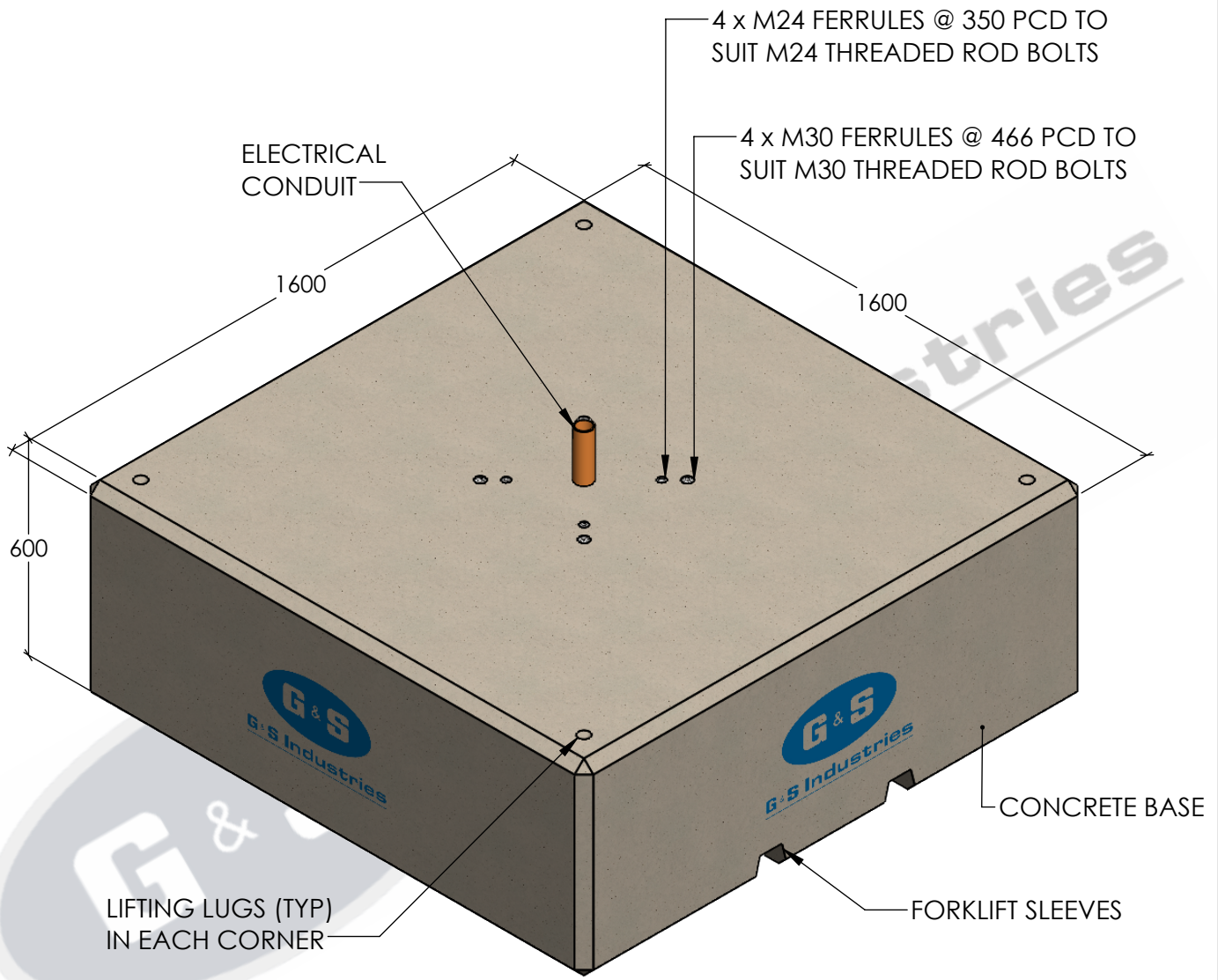
3D VIEW SCALE 1:15
