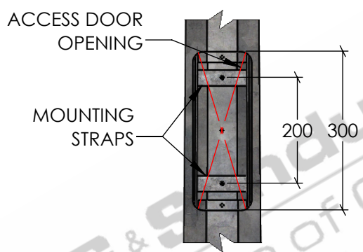
*DOOR REMOVED FOR CLARITY ELEVATION ON DOOR SCALE 1:10
