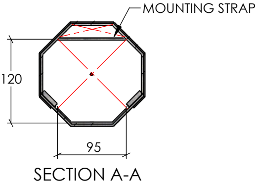
SECTION A-A ACCESS DOOR CLEARANCE DETAIL SCALE 1:5
