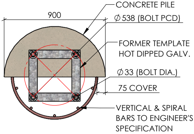
TOP VIEW SCALE 1:20
