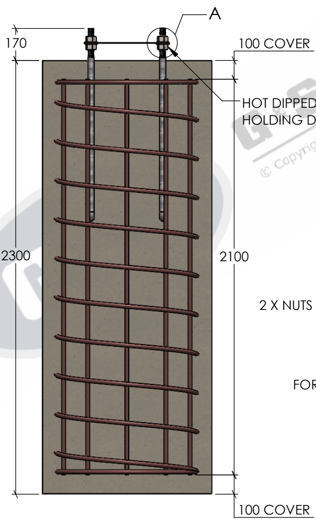
SIDE ELEVATION SCALE 1:30
