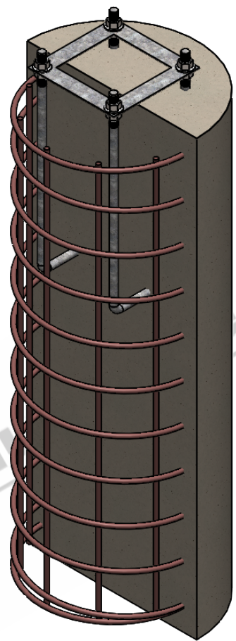
ISOMETRIC ELEVATION SCALE 1:30
