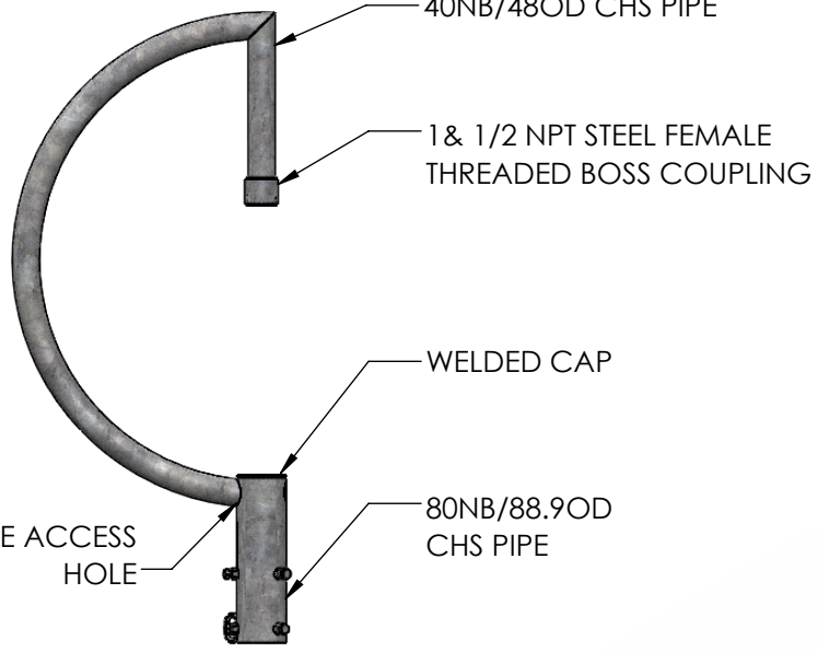
SIDE ELEVATION 2 SCALE 1:15
