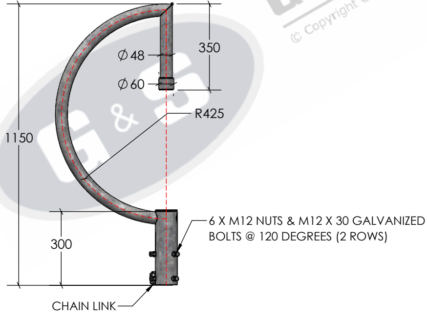
SIDE ELEVATION 1 SCALE 1:15
