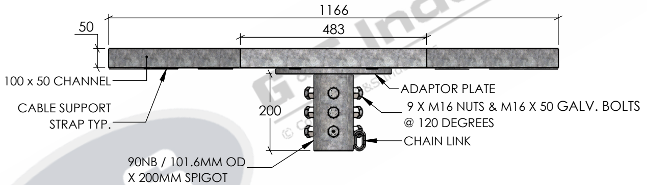
ISOMETRIC VIEW
