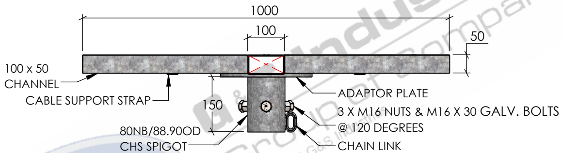
ISOMETRIC VIEW
