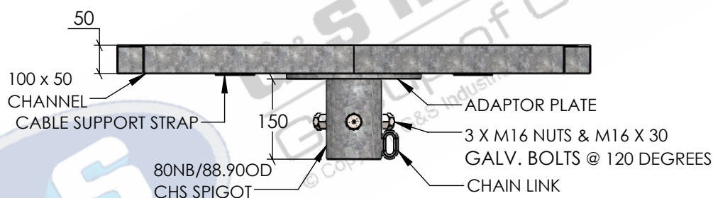
ISOMETRIC VIEW
