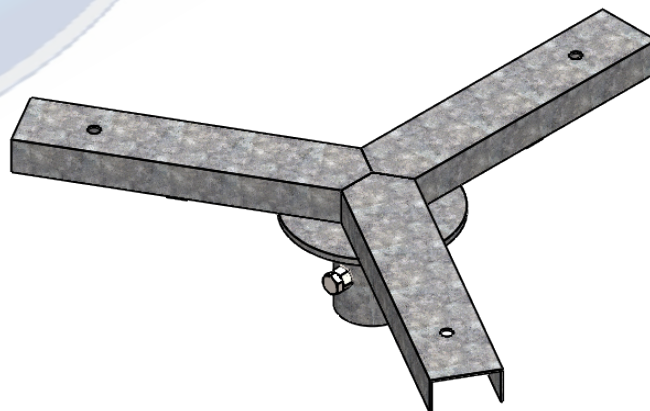
ISOMETRIC VIEW
