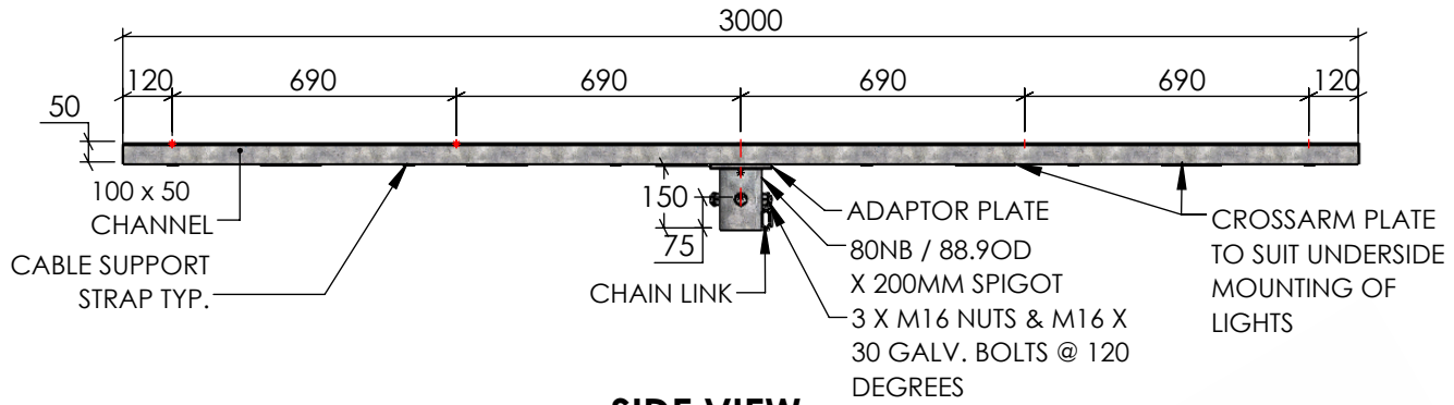
SIDE VIEW SCALE 1:15
