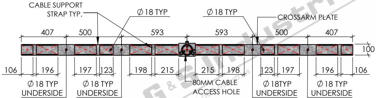
BOTTOM VIEW SCALE 1:15
