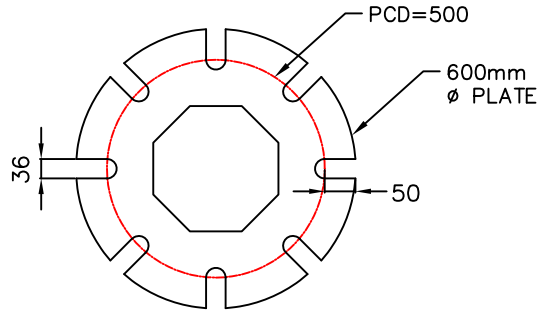
BASEPLATE THICKNESS: 40mm BASEPLATE DETAILS
