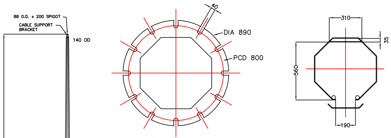
BASEPLATE THICKNESS: 32mm BASEPLATE DETAILS
