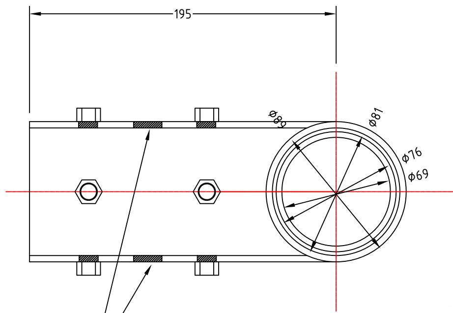
M18 HOLE THROUGH BOTH SIDES OF PIPE TOP VIEW
