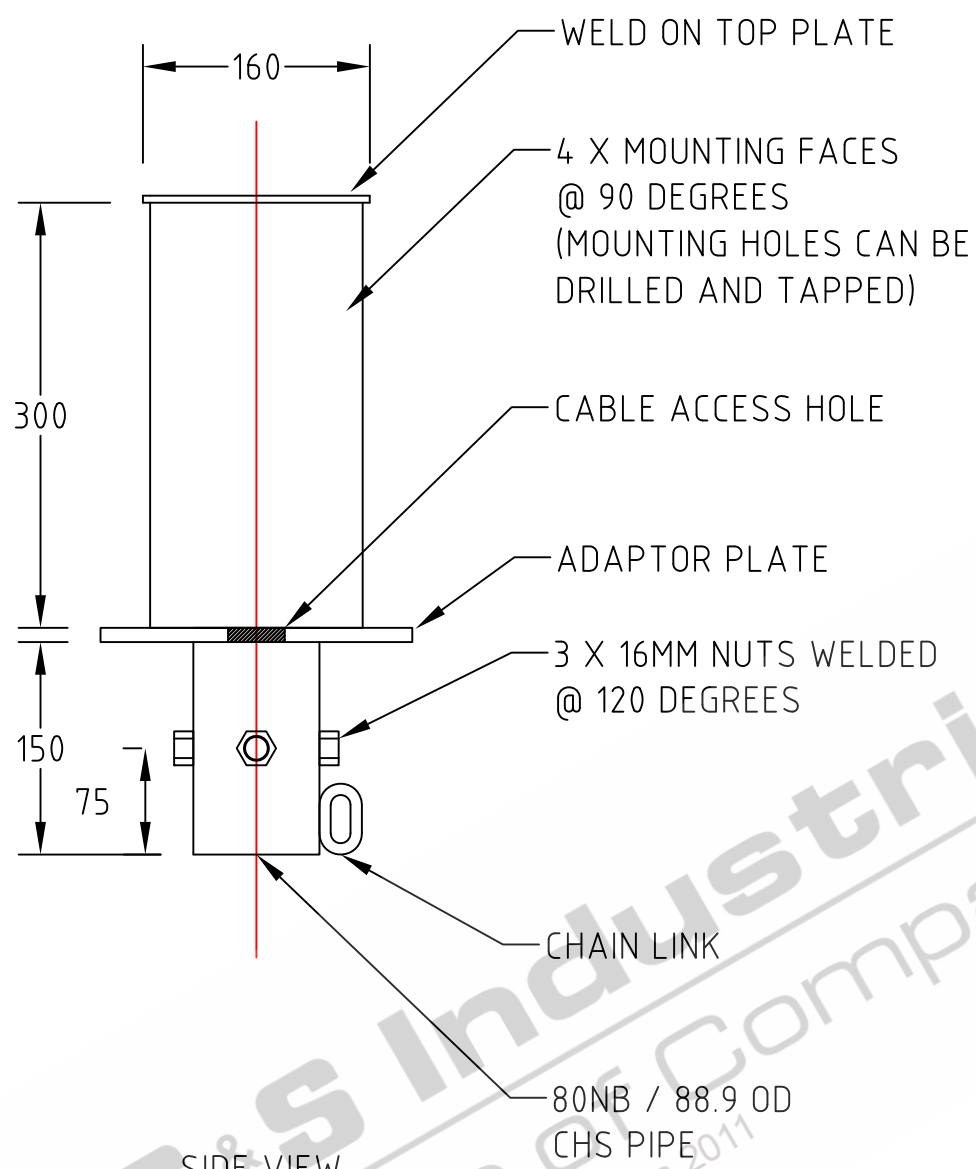
SIDE VIEW
