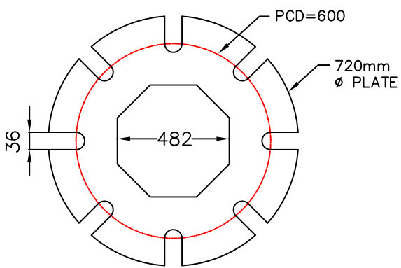
BASEPLATE THICKNESS: 40mm BASEPLATE DETAILS
