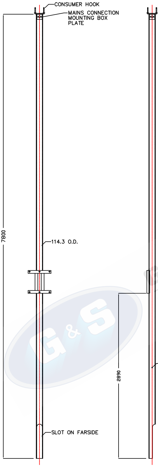
FRONT VIEW
